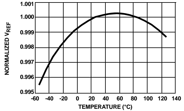
FIGURE 2. REFERENCE VOLTAGE vs TEMPERATURE
