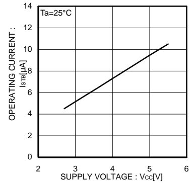
Fig.5 Standby Current AEN Disable
