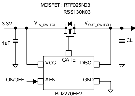
Fig.31 Switch Rise / Fall Characteristics Measurement Circuit Diagram
