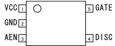
Fig.33 Pin Configuration
