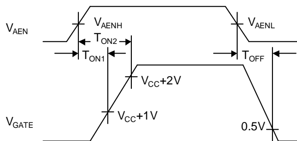
Fig.2 Timing Diagram
