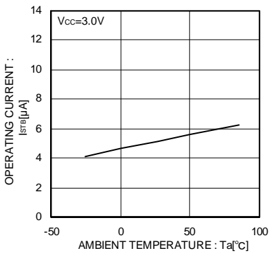
Fig.6 Standby Current AEN Disable
