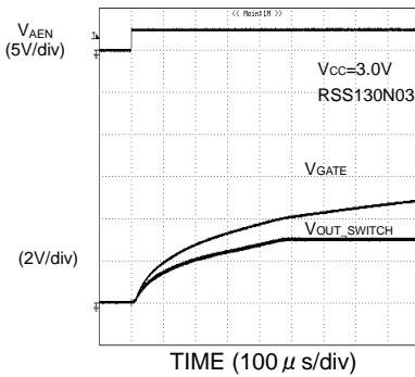
Fig.29 GATE Switch Rise Characteristics
