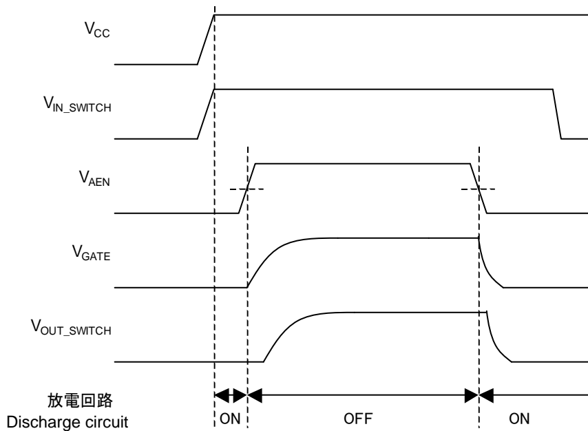
Fig. 34 Operation Timing
