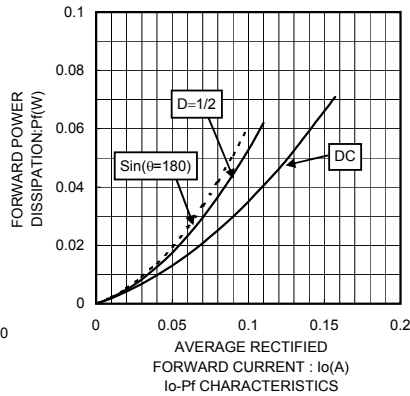
AVERAGE RECTIFIED FORWARD CURRENT : Io(A) Io-Pf CHARACTERISTICS
