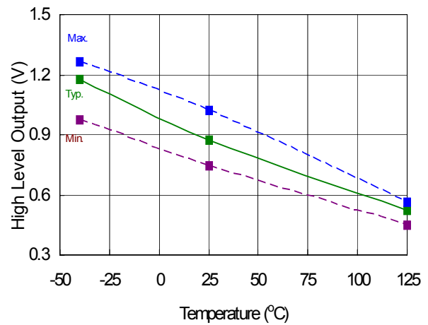
Figure 5. High Level Output Voltage vs. Temperature (Io = 0mA)
