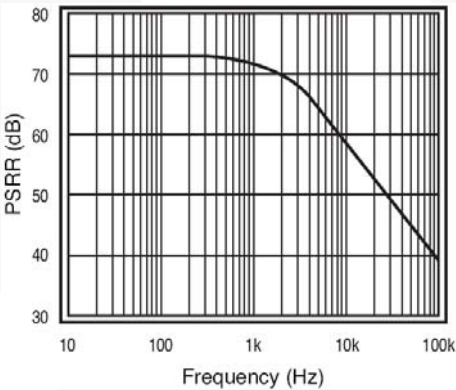
Figure 16. PSRR V_S=5V
