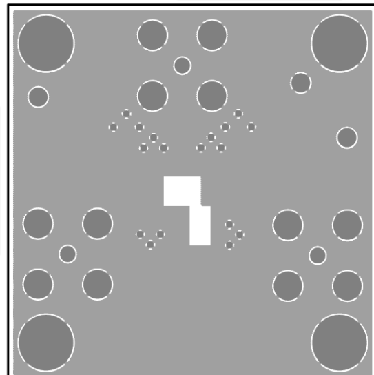
Figure 26. Bottom Side
