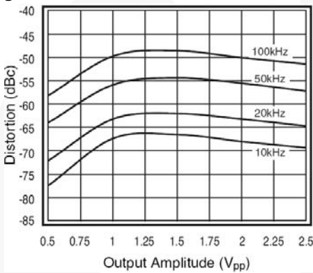
Figure 14. 3rd Harmonic Distortion vs. V_o
