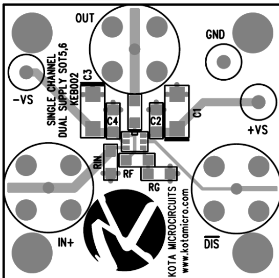
Figure 25. Top Side
