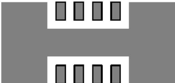
Copper Area = 70\text{mm}^2 , \theta_{JA} = 49^{\circ}\text{C/W}
