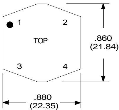
Physical Dimensions inches (mm)
