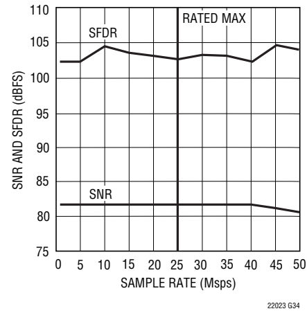
LTC2203: SNR and SFDR vs Sample Rate
