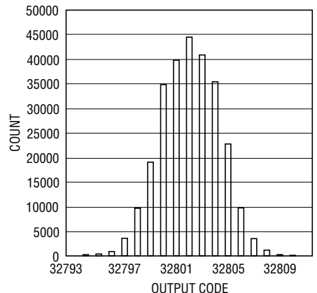
LTC2202: AC Grounded Input Histogram (256K Samples)
