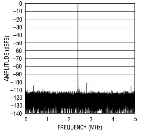
LTC2202: 32K Point FFT, f_{IN} = 12.4\text{MHz} , -1\text{dBFS} , \text{PGA} = 0
