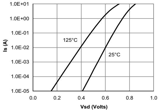
Figure 6: Body-Diode Characteristics
