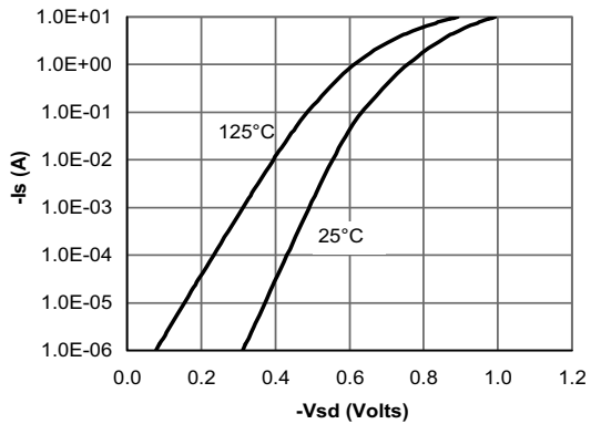
Figure 6: Body-Diode Characteristics
