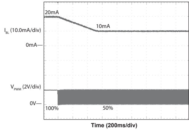
I_{BL} Settling Time — 100% to 50%
