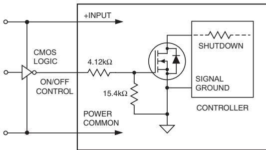
Figure 2A. Inverting On/Off Control Pin with an External CMOS Gate
