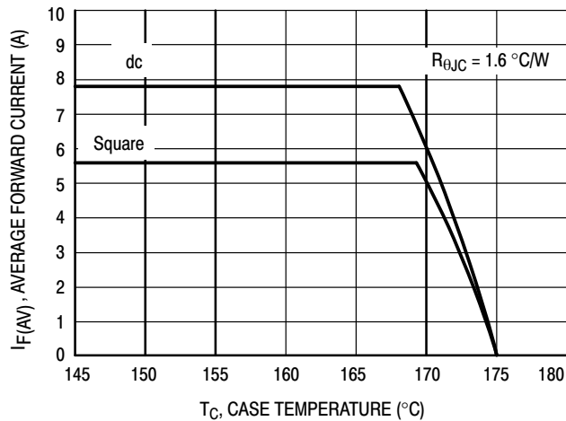
Figure 6. Current Derating, Case
