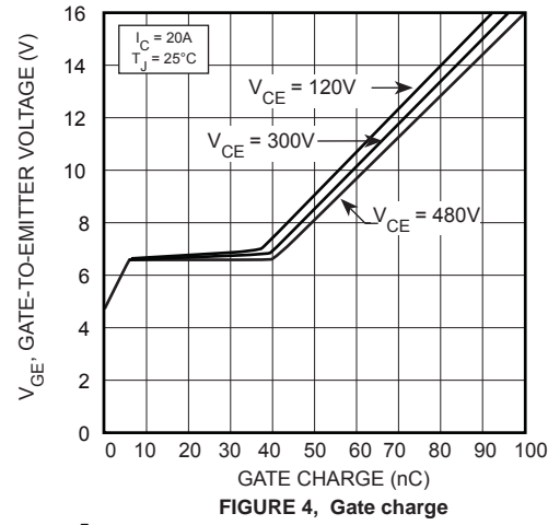
FIGURE 4, Gate charge
