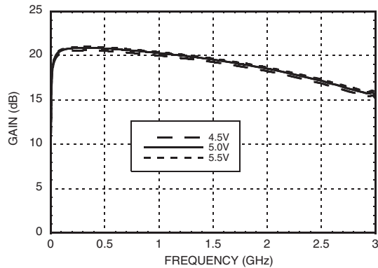
Gain vs. Vcc
