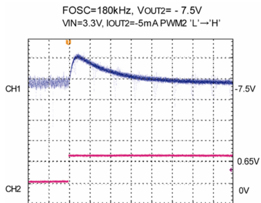
200 \mu sec/div CH1:VOUT2 , AC-COUPLED ,20mV/div CH2:PWM2 , 0.5V/div
