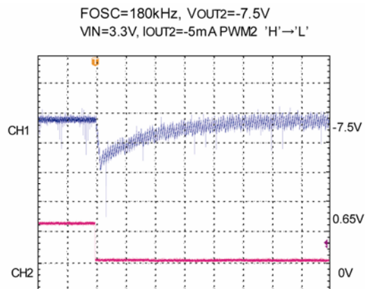
200 \mu sec/div CH1:VOUT2, AC-COUPLED ,20mV/div CH2:PWM2, 0.5V/div
