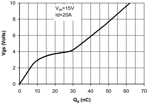
Figure 7: Gate-Charge Characteristics
