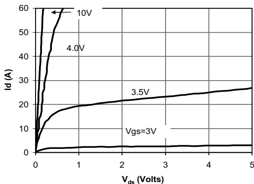
Fig 1: On-Region Characteristics
