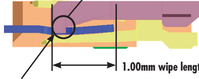
FPC lock for secure cable retention
