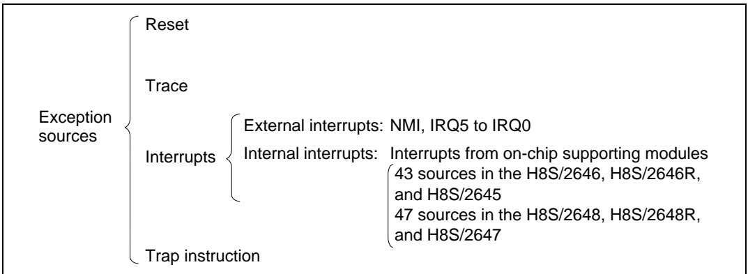
Figure 4.1 Exception Sources
