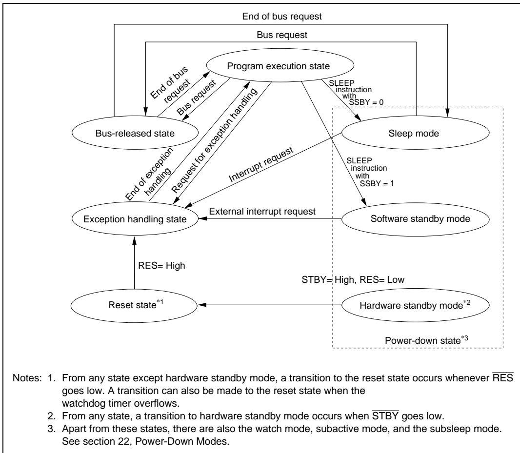
Figure 2.15 State Transitions
