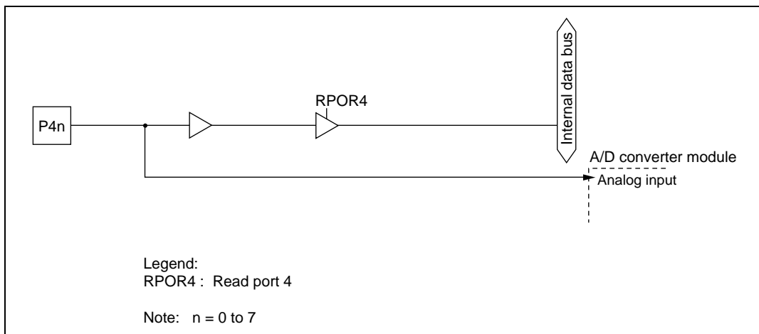
Figure C.4 Port 4 Block Diagram (Pins P40 to P47)
