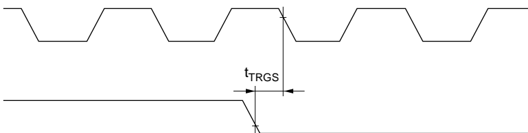
Figure 23.19 A/D Converter External Trigger Input Timing
