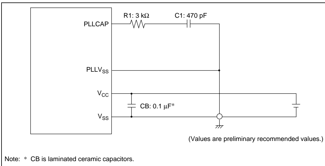
Figure 21.5 Points for Attention when Using PLL Oscillation Circuit
