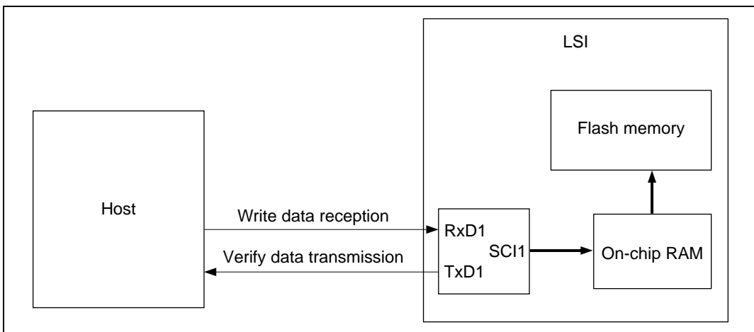
Figure 20.6 System Configuration in Boot Mode
