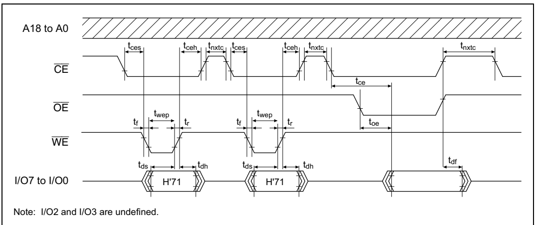
Figure 21C-24 Status Read Mode Timing Waveforms
