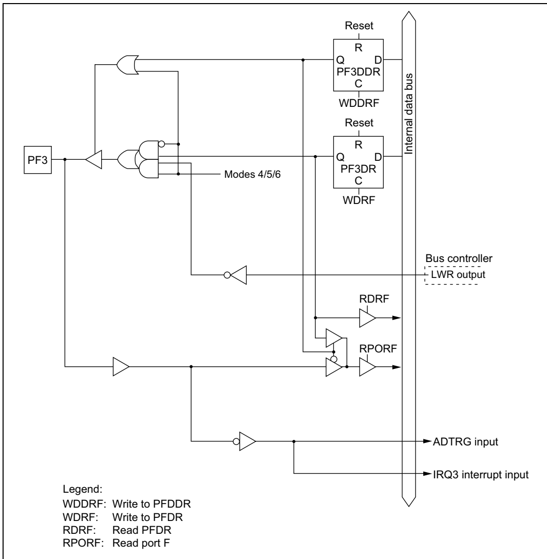
Figure C-10 (b) Port F Block Diagram (Pin PF3)
