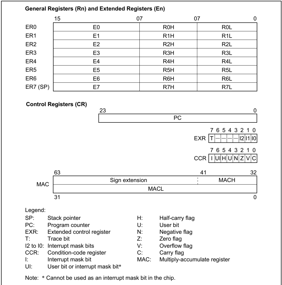
Figure 2-7 CPU Registers
