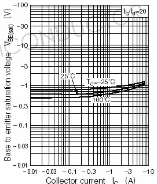
Fig.6 Base-Emitter Saturation Voltage
