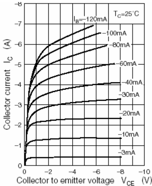
Fig.3 Static Characteristic
