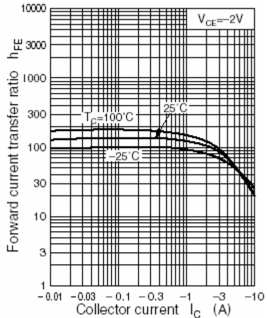
Fig.4 DC current Gain
