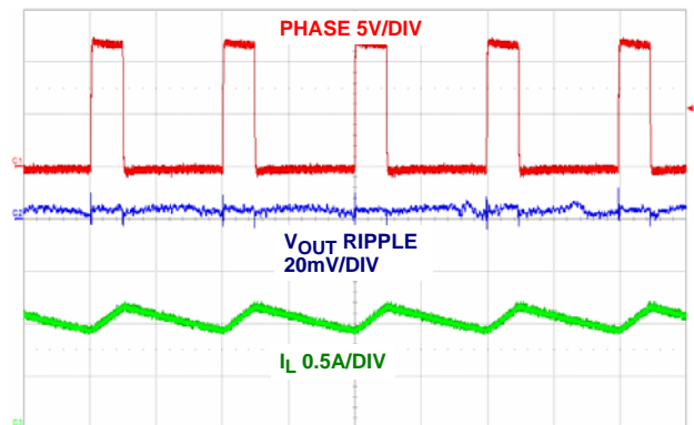
FIGURE 13. STEADY STATE OPERATION AT FULL LOAD (1µs/DIV)
