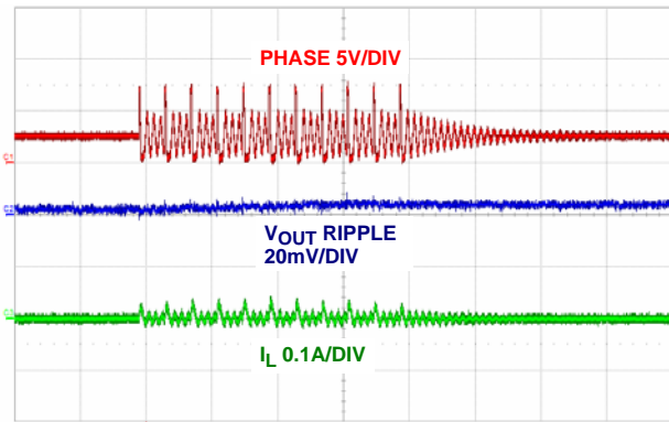
FIGURE 12. STEADY STATE OPERATION AT NO LOAD (5µs/DIV)
