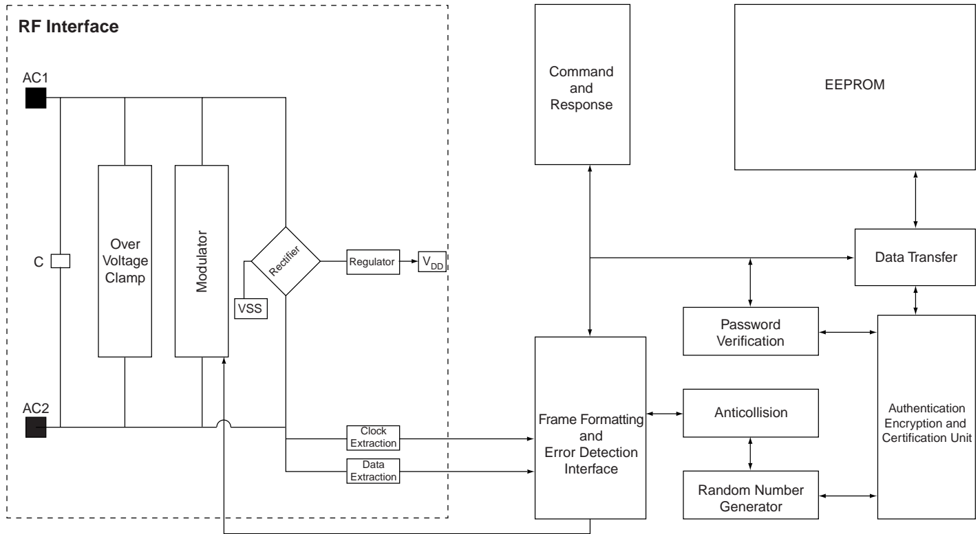
Figure 1. Block Diagram
