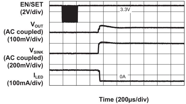
Movie Mode Current Transition
