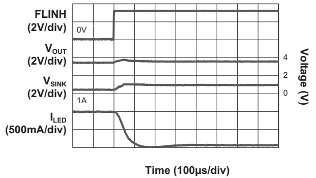
Flash Inhibit On Delay Time (EN/SET = 0V; FLEN = 3.3V; 500mA/ch)
