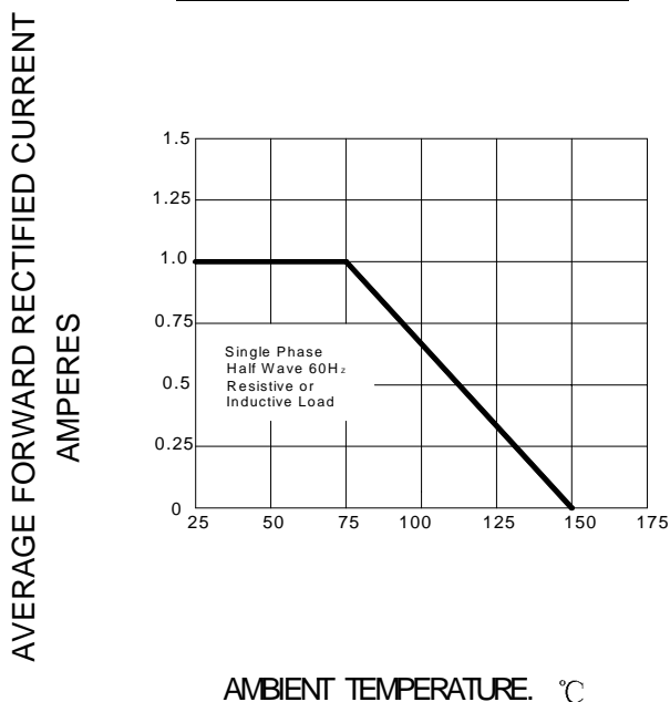
FIG.3 – FORWARD DERATING CURVE
