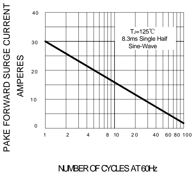
FIG.5 – PEAK FORWARD SURGE CURRENT
