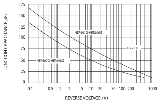
FIG.6-TYPICAL JUNCTION CAPACITANCE
