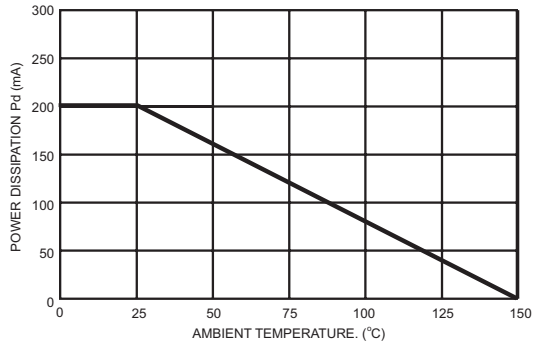
FIG.2- DERATING CURVE
