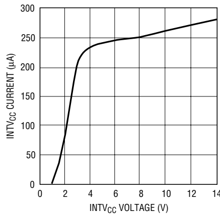
INTV CC Shutdown Current vs INTV CC Voltage
