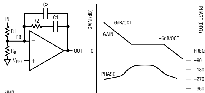
Figure 11. Type 2 Schematic and Transfer Function
