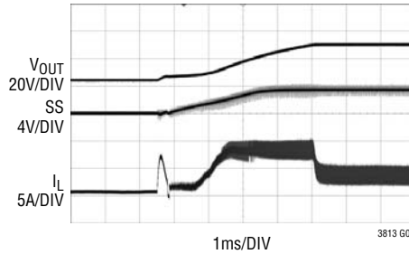
FRONT PAGE CIRCUIT V_{IN} = 24V I_{LOAD} = 2A
