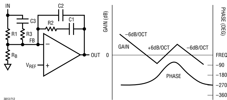
Figure 12. Type 3 Schematic and Transfer Function
