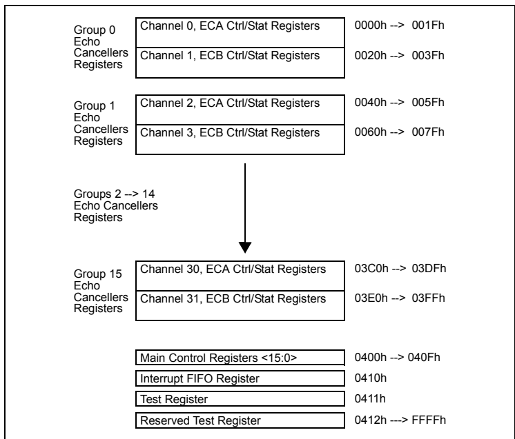
Figure 10 - Memory Mapping
