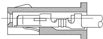
TERMINAL ASSEMBLY DRAWING
