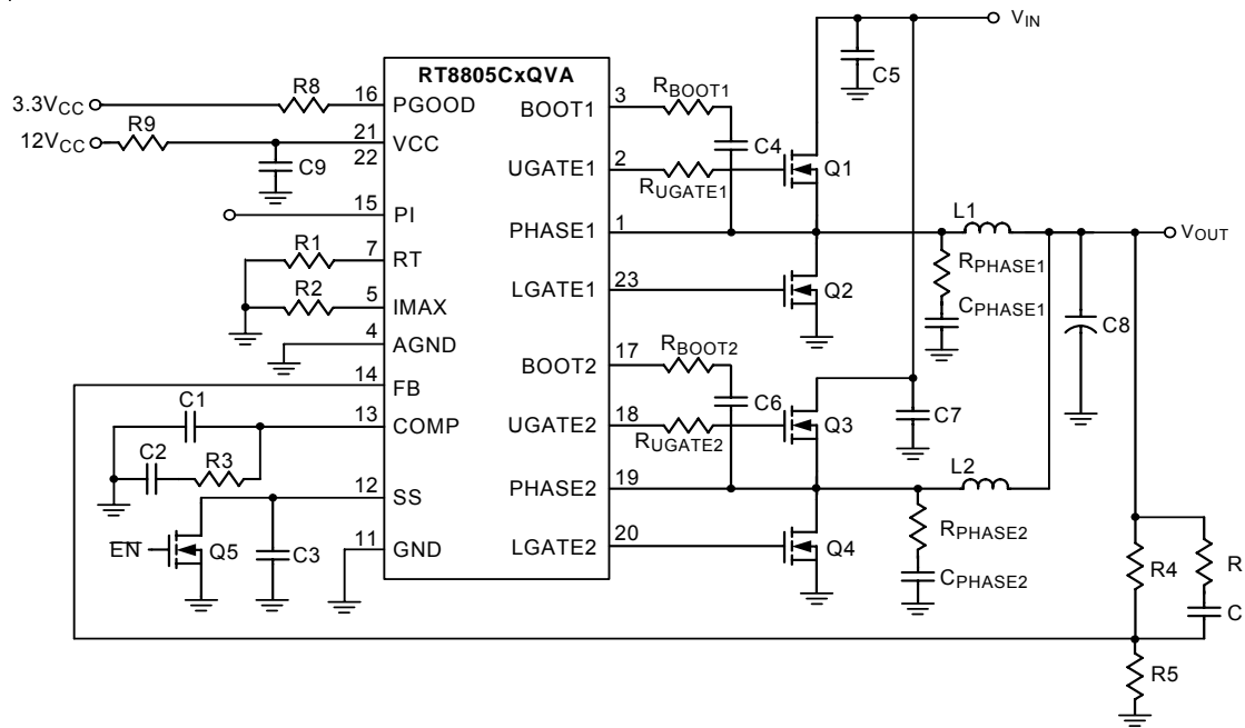
Figure B. Application Circuit for RT8805CxQVA (VQFN-24L 4x4)-Standalone Mode (PI Disabled)
