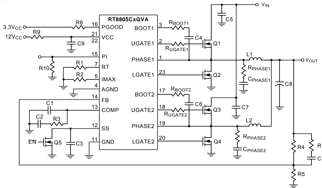
Figure C. Application Circuit for RT8805CxQVA (VQFN-24L 4x4)-Tracking Mode (PI Enabled)
