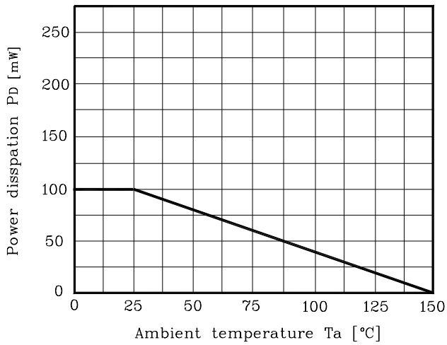
Fig9 P_D - T_a
