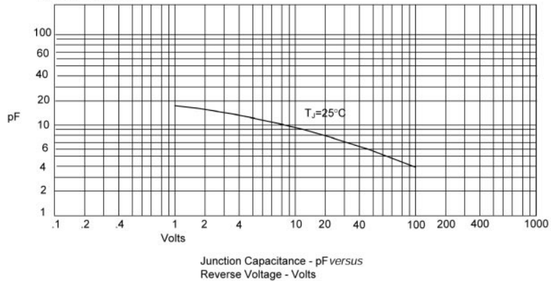
Figure 3 Junction Capacitance
