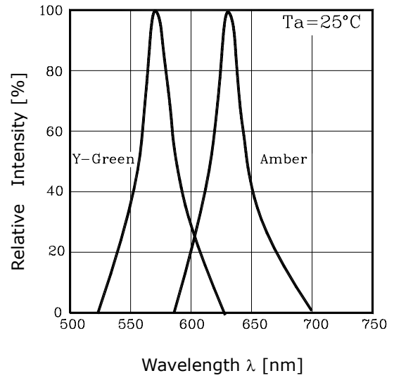
Fig. 4 Spectrum Distribution
