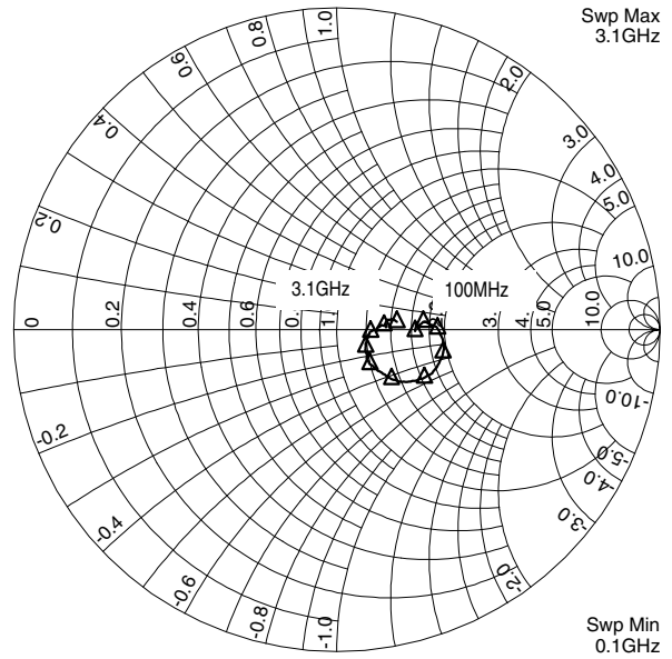
RF2322 S22, Vcc = 2.7 V, Temp = 25°C
