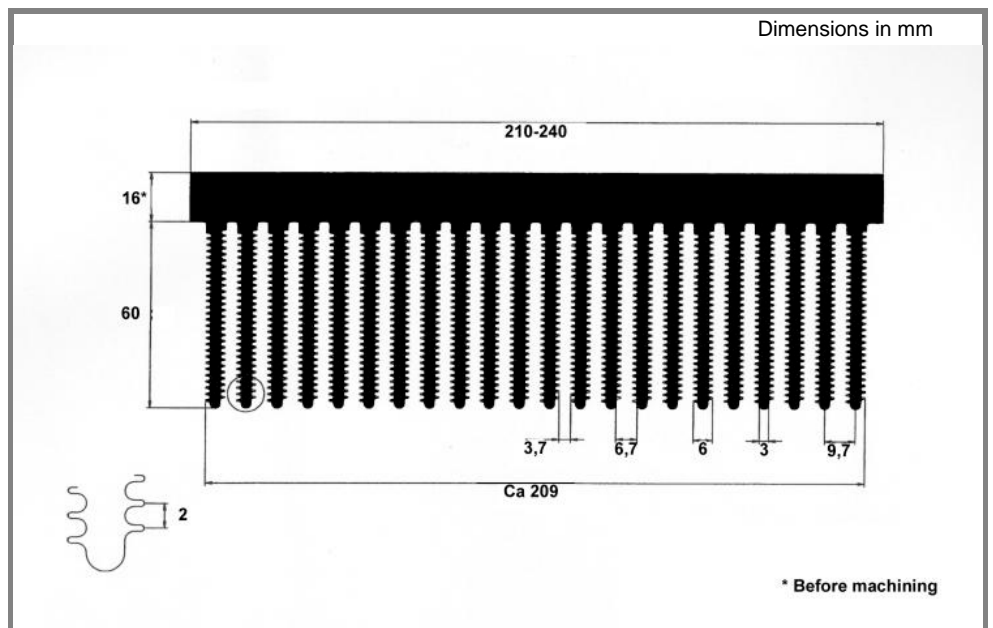
Px 16 general profile dimensions (w = 26,6 kg/m)
