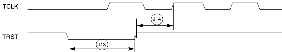
Figure 27. TRST Timing
