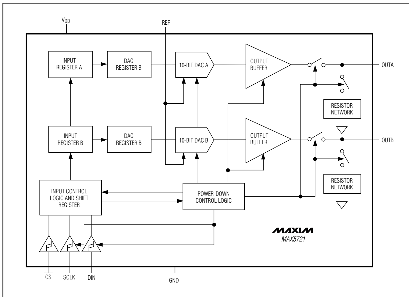
Functional Diagram
