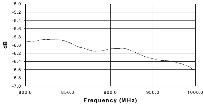
Conversion Loss
