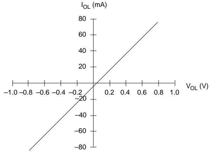
Output, LOW
