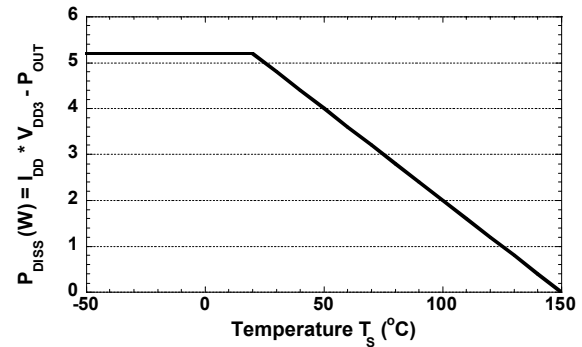
Maximum Operating Temperature ( T_s ) to Maintain <150^\circ\text{C} Junction Temperature.
