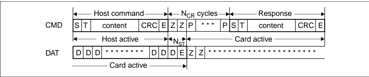
Timing of Stop Command (CMD12, Data Transfer Mode)
