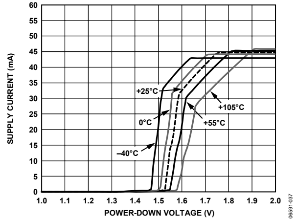
Figure 38. Supply Current vs. \overline{PD} for Various Temperatures, V_s = 3.3 V
