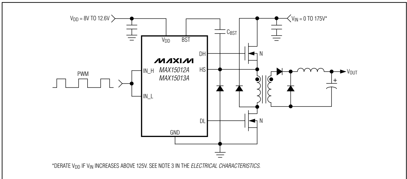
Figure 3. Two-Switch Forward Conversion
