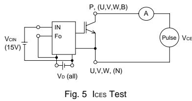
Fig. 5 ICES Test
