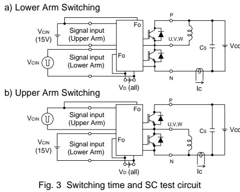
Fig. 3 Switching time and SC test circuit
