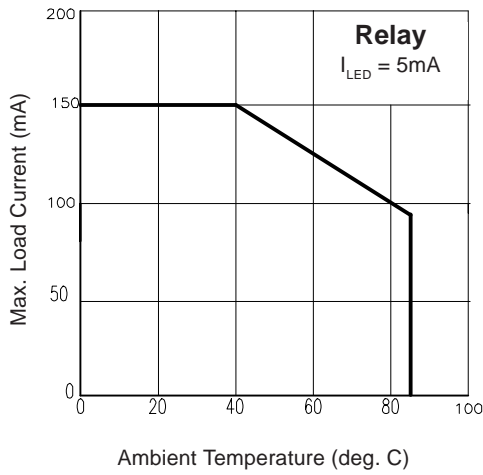
Figure 1. Current Derating Curve
