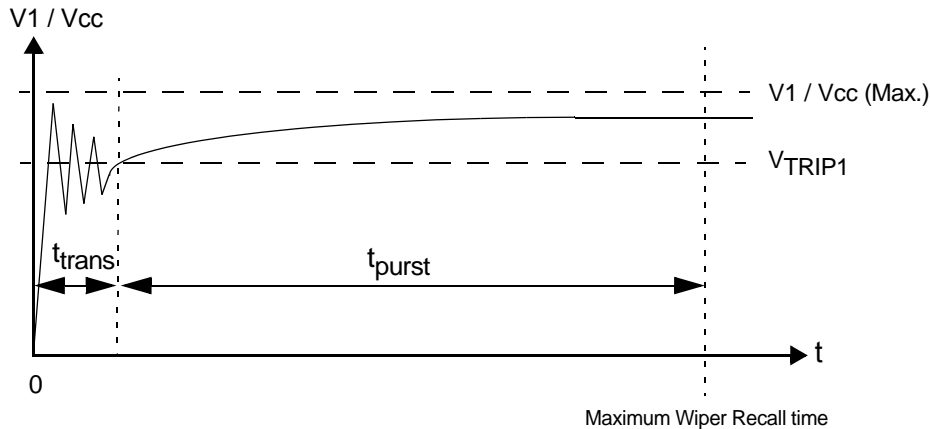
Figure 7. DCP Power
