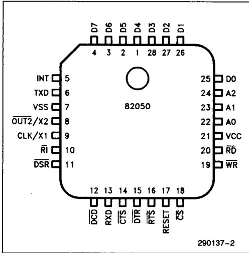
Figure 2. PLCC Pinout
