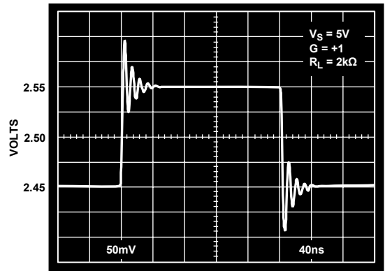
Figure 38. AD8054 100 mV Step Response; V_S = 5\text{V} , G = +1
