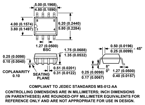
Figure 56. 8-Lead Standard Small Outline Package [SOIC_N] Narrow Body (R-8)
