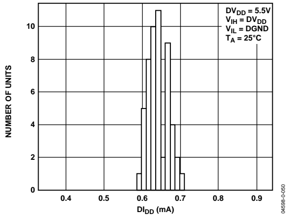
Figure 16. D_{lDD} Histogram
